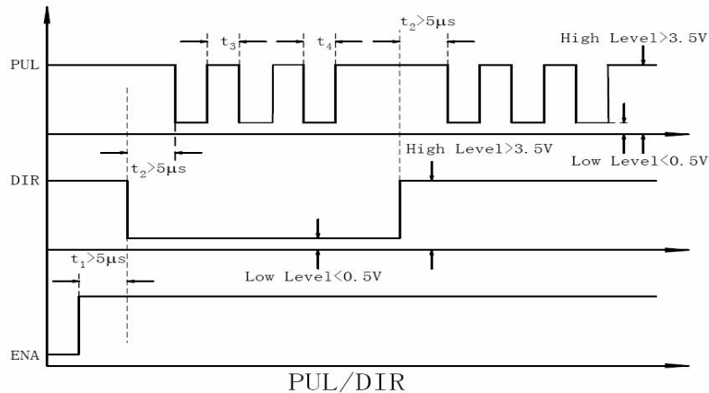
Figure 5: Sequence chart of control signals
