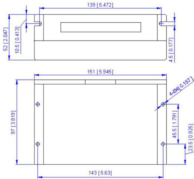
Figure 1: Installation specifications
